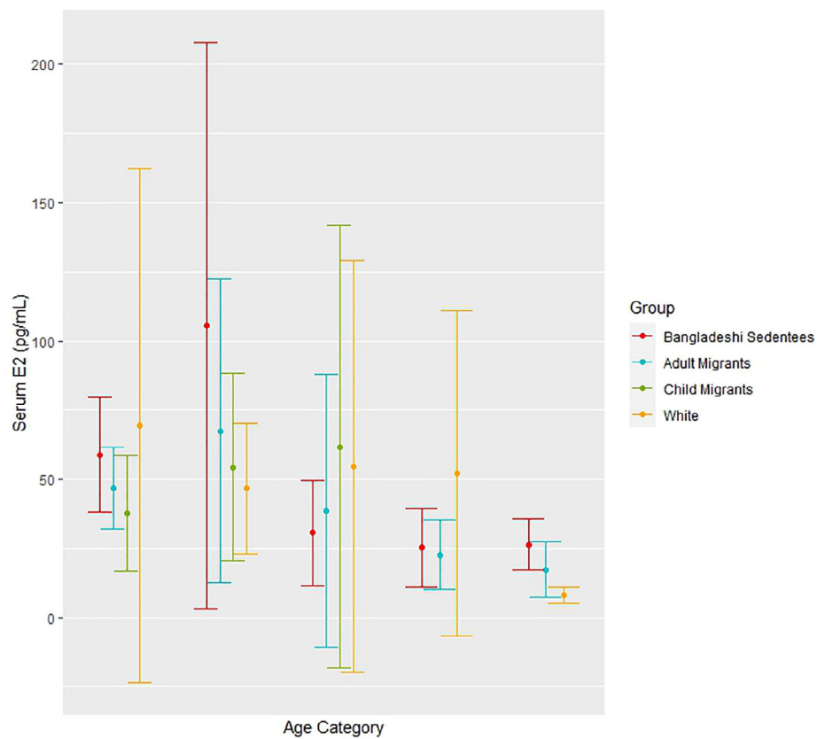
FIGURE 1 Serum estradiol (E2) levels (pg/ml) across the reproductive lifespan. Error bars represent the SD. Age categories: 1 = 35–39 ( n = 55 ); 2 = 40–44 ( n = 40 ); 3 = 45–49 ( n = 33 ); 4 = 50–54 ( n = 26 ); 5 = 55–59 ( n = 24 )
